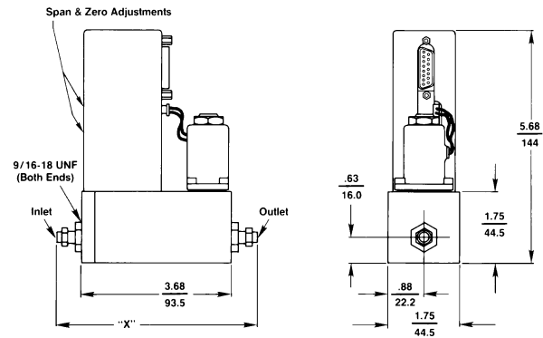
5851E/5851i, 15-Pin D Connector
